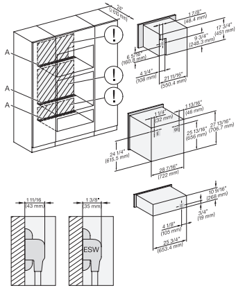
DGC7x4x+EBA7848, H2880BP, H7x6xBP(X), ESW7x80, Installation, 30 Zoll, Proud, combi, XL, 650
