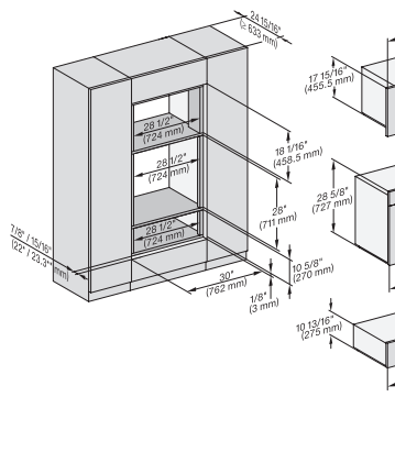
H 6x80 BP, H 6x00 BM + EBA 6808, ESW 6x80, DGC 6x00-1, H 6x80-2BP, DGC7x40, EBA 7848, H2880BP, H7x80BP, Flush inset, NA
