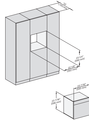
installation Proud 650S, installation drawing, NA
