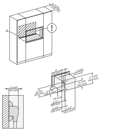
installation 30 inch Flush inset DGC30 XL, installation drawing, NA
