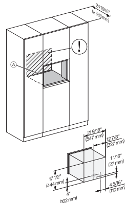
CVA7445, CVA7845, installation drawing, 60 cm, Flush insert
