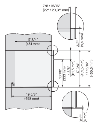
CVA7445, CVA7845, side view, 60 cm, Proud insert
